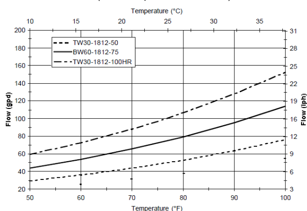
Figure 3: Impact of temperature on permeate flow (constant pressure, recover)
