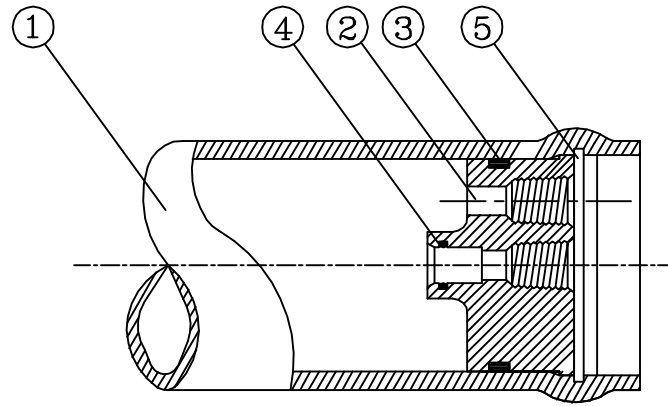
SECTION THROUGH END CLOSURE
